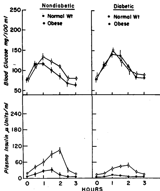
FIG. 4. PLASMA INSULIN RESPONSES OF 15 NORMAL, 12 OBESE NONDIABETIC, 12 NORMAL WEIGHT DIABETIC, AND 12 OBESE DIABETIC SUBJECTS TO INFUSION MAINTAINED NORMAL BLOOD GLUCOSE PROFILE. Values represent mean \pm SEM.
