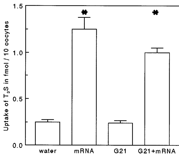
FIG. 6. Initial uptake of T 3 S in X. laevis oocytes injected with water (control), fractionated rat liver mRNA, cRNA for rat liver type 1 deiodinase (G21), or both (G21 + mRNA). Values are means ± SEM; *, P < 0.001 vs. water. [Modified reproduction with permission from R. Docter et al. : Endocrinology 138:1841–1846, 1997 (197). © The Endocrine Society.]
