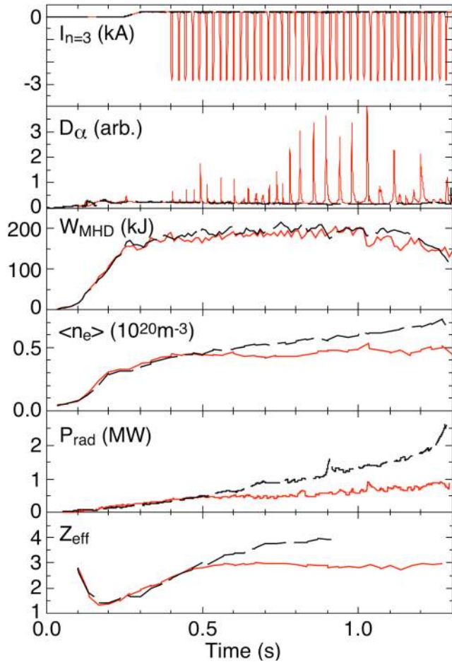
Figure 9. Comparison of similar discharges without (black dashed) and with (red solid) the application of a train of pulses in the error-field correction coils to create an n = 3 magnetic perturbation. The pulses trigger repeated ELMs which have been suppressed by the lithium coating. The ELMs have little effect on the stored energy, but reduce the volume average density, radiated power and average Z_{\text{eff}} .
