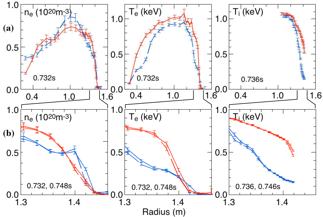
Figure 3. (a) Full radial profiles of the electron density and electron and ion temperature measured close to the time of peak stored energy for the discharges in Fig. 2; (b) Details of the profiles in the outer edge region for two successive Thomson scattering measurement times showing the changes in the edge after lithium coating.
