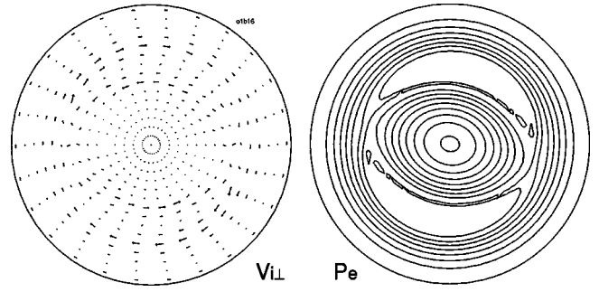
FIG. 2. Profiles with steady state, bootstrap current driven neoclassical magnetic islands. The left figure shows that the perpendicular flow of ion fluid vanishes except near the island region, as expected in this \nabla T = 0 case. The islands (shown here as flat electron pressure regions) rotate with \omega \approx 0.3\omega_e^* in the lab frame, and \omega \approx 0.7\omega_e^* in the guiding center frame. Without the neoclassical effects, the islands are fixed in the guiding center frame.
