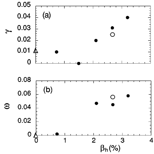
FIG. 4. (a) Growth rates, and (b) rotation frequencies of m=1 internal modes at various \beta_h values of the fusion alphas, obtained from MHD (triangles), from the gyrokinetic-energetic-particle/MHD hybrid model (solid circles), and from the gyrokinetic-particle-ion/fluid-electron hybrid model (open circles).
