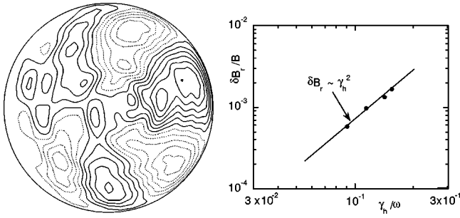
FIG. 3. The left figure shows the stream lines of the incompressible part of the velocity in a nonlinearly saturated TAE mode. The saturation mechanism is found to be wave-particle trapping. The right figure shows the saturation amplitude as a function of the growth rate, and agreement with the analytic prediction.
