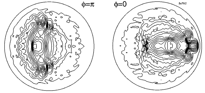
FIG. 1. Pressure contours during a high- \beta disruption for a reversed shear plasma. Nonlinear development of a ballooning mode produces pressure steepening in the normal shear region with a structure which looks like fingers in 2D and ribbons in 3D. This can cause magnetic field line stochasticity and a thermal quench.
