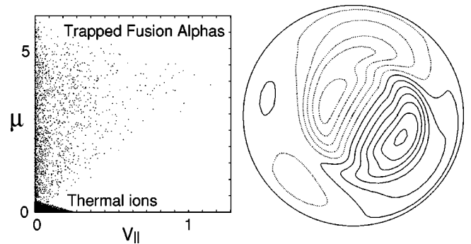
FIG. 5. The profiles of the case corresponding to the open circles in Fig. 4. The magnetic moment \mu versus v_{\parallel} plot on the left shows the trapped part of the slowing down fusion alphas, and thermal ion particles with a temperature 0.01 times the alpha temperature. A quarter million particles each are used to represent the alphas and thermal ions. The figure on the right shows the stream lines of the incompressible part of the mass flow.
