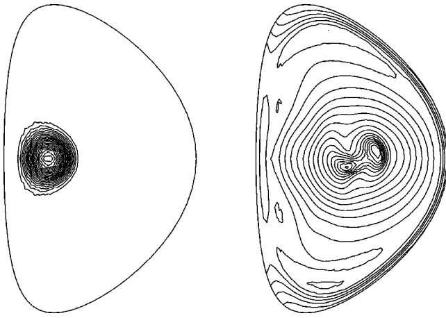
FIG. 6. Density contours showing an inboard-side injected pellet. The pellet can penetrate deep into the plasma, accompanying a reconnection process as shown on the right.
