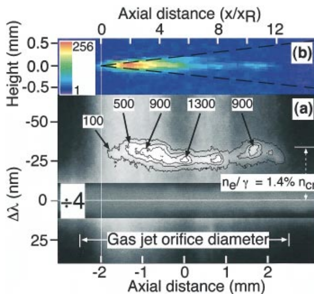
FIG. 3(color). Results from two imaging diagnostics from the same laser shot with P \approx 20 TW and n_c/\gamma \approx 1.4 \times 10^{19} cm -3 . Axial distance represents position along the laser axis. (a) Time-integrated (20 ps probe pulse and 1/2 ns optical gate) raw-data image from collective Thomson scattering. Contours of constant scattered energy were obtained by subtracting the average bremsstrahlung background at each spatial location and applying the contours to the resultant Thomson-scattering-only image. The effective plasma density is labeled in terms of the critical density ( n_{cr} ) for the pump frequency. Stray light near \Delta\lambda = 0 was divided by 4 in the image file. (b) (color) Side-view sidescatter image dominated by light near 1 \mu\text{m} . Dashed lines represent the f/4.5 focal cone of the laser in vacuum.
