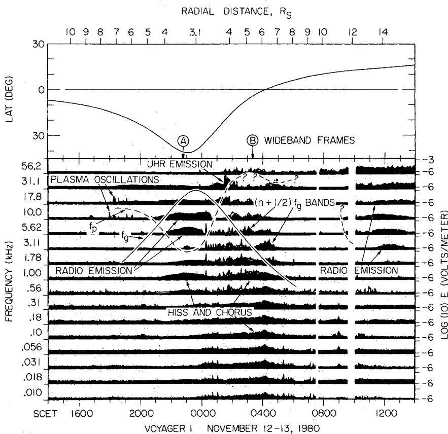
Fig. 3 (right). The plasma wave electric field intensities in the region near closest approach. The dashed line gives the approximate electron plasma frequency ( f_p ) profile derived from a combination of electron plasma oscillations, radio emission propagation cutoffs, and UHR emissions. Question marks indicate regions of uncertainty in the profile. The electron gyrofrequency ( f_g ) profile was obtained from the magnetometer. Arrows marked A and B refer to spectrograms in Fig. 5.
