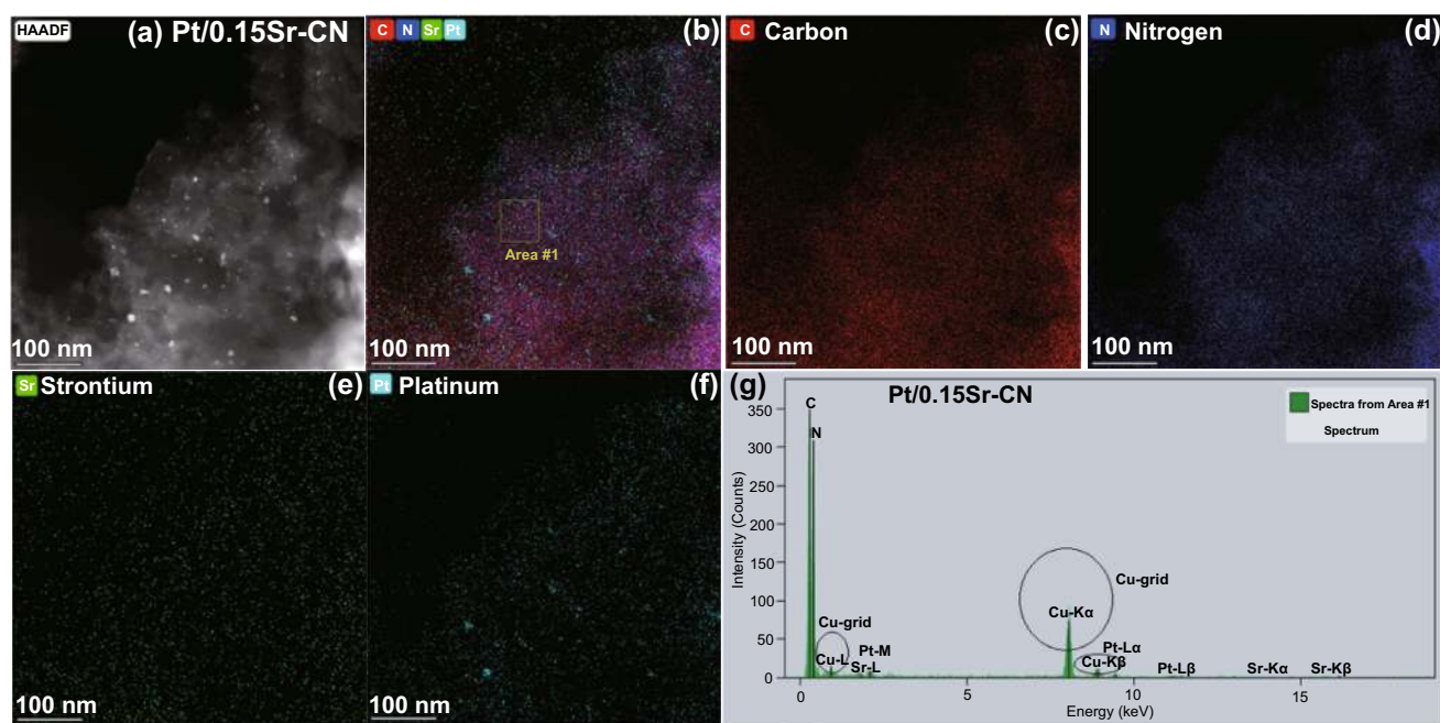
Fig. 4 TEM mappings of a, b Pt/0.15Sr-CN, c carbon element, d N element, e Strontium element, and f Platinum. g EDX spectrum of Pt/0.15Sr-CN
