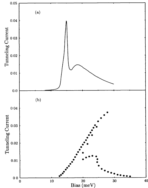
FIG. 4. (a) Plot of tunneling current as a function of applied bias; the current is expressed in units of en_e(2E_e/m)^{1/2} , where n_e is the charge density in the emitter and E_e is the energy level of the emitter. (b) Same as (a) but with the electron feedback effect in the resonant well.
