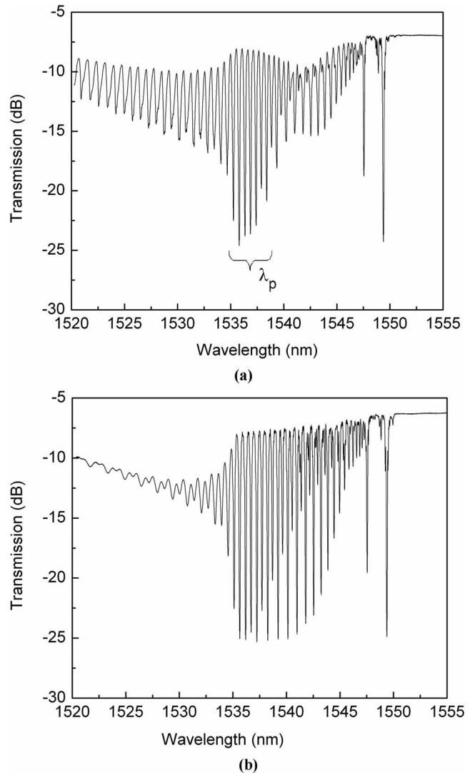
Fig. 3. (a). Transmission spectrum of the same grating as in Fig. 1 but with a 20 nm gold coating and immersed in a sucrose solution with n_D=1.4378 . The bracket indicates the peak position of the anomalous resonance. (b) Same as (a) but without the gold film.
