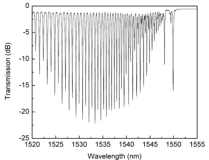
Fig. 1. Transmission spectrum of a weakly tilted FBG.
