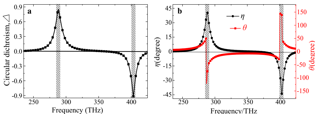
Fig. 3 The calculated relative optical parameters of the proposed CMSA for the normal incident LCP and RCP lights, a the CD parameter \Delta , b ellipticity angle \eta and polarization azimuth rotation angle \theta
