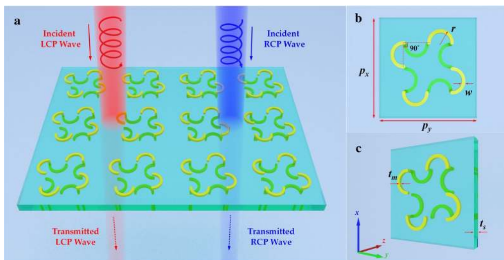
Fig. 1 Schematic of the designed CMSA: a periodic array, b, c the front and perspective view of the unit-cell nanostructure. The periodic lengths along x - and y -axis directions are both 600 nm, and the normal incident CP lights are propagating along the z -axis direction
