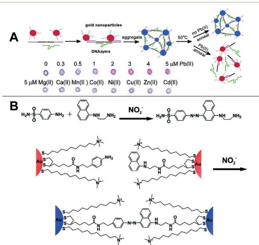
Fig. 3 A) DNAzyme-directed assembly formation and cleavage of gold nanoparticles in a \text{Pb}^{2+} colorimetric sensor, 102 Reprinted with permission from J. Liu and Y. Lu, J. Am. Chem. Soc. , 2003, 125 , 6642–6643. Copyright 2014 American Chemical Society. B) Schematic of the Griess reaction and Griess reaction induced aggregation of AuNPs. 14 Reprinted with permission from W. L. Daniel, M. S. Han, J. S. Lee and C. A. Mirkin, J. Am. Chem. Soc. , 2009, 131 , 6362–6363. Copyright 2014 American Chemical Society.
