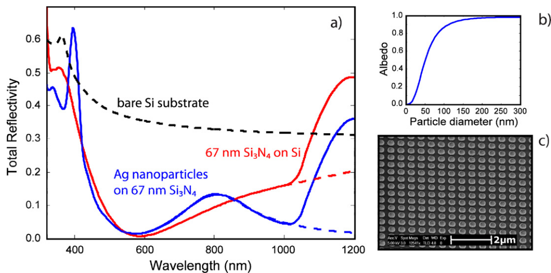
Figure 4. (a) Measured total reflection spectrum from a 300 \mu\text{m} crystalline Si cell coated with 67 nm Si 3 N 4 (red) and the same sample with an optimized Ag particle array on top (blue). The particles reduce the reflection for wavelengths above 800 nm, improving the coupling of light into the Si substrate. The dashed lines are extrapolated data representing the reflection from a semi-infinite substrate. The calculated reflectance of a semi-infinite Si substrate is shown for reference (dashed black line). (b) Calculated albedo of a silver nanoparticle in air as a function of particle diameter. (c) An SEM image of the optimal Ag nanoparticle arrays. Figures reproduced with permission: ©ACS (2011).
