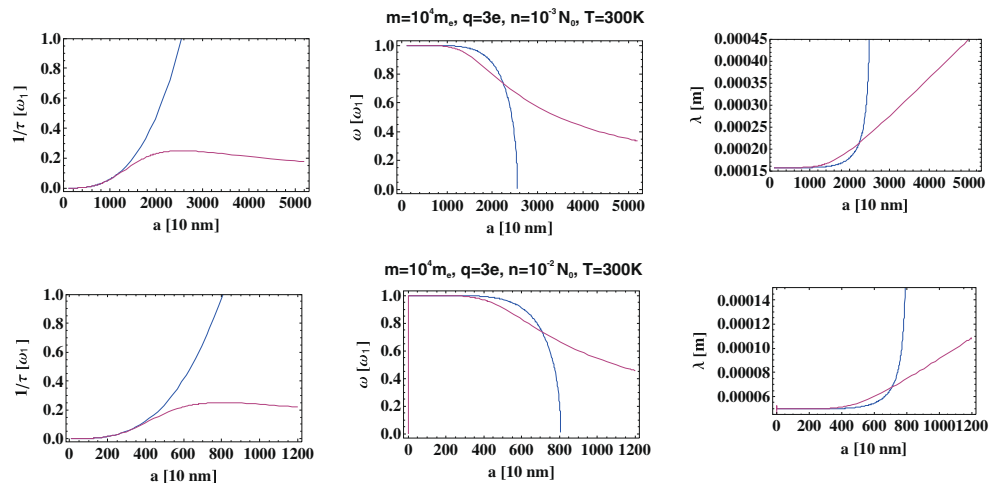
Fig. 4 Comparison of the damping rate and the resonance frequency (the latter expressed in the right panel by the resonance wavelength), i.e., the damping rate and frequency (wavelength) of the oscillating solution of Eq. 35, exact one (given by Eq. 36—red line) and perturbation approximation (given by Eq. 34—blue line), both with respect to the finite ionic system radius a
