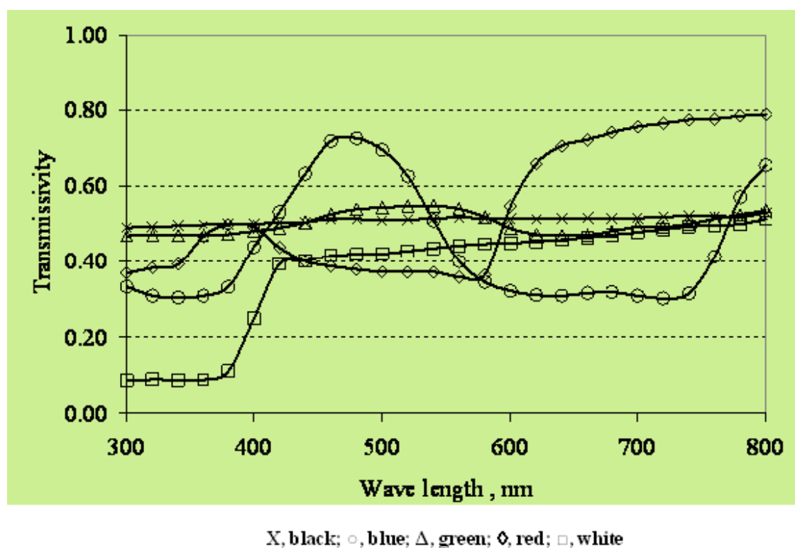
Figure 3. Diagram of transmissivity measured in 300- to 800-nm wave length range on different colored nets tested in laboratory.
