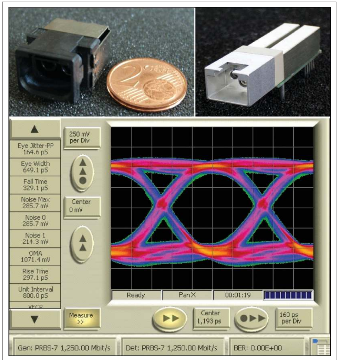
■ Figure 4. Gb/s transceiver modules and eye diagram of a 50 m GI-POF link.
