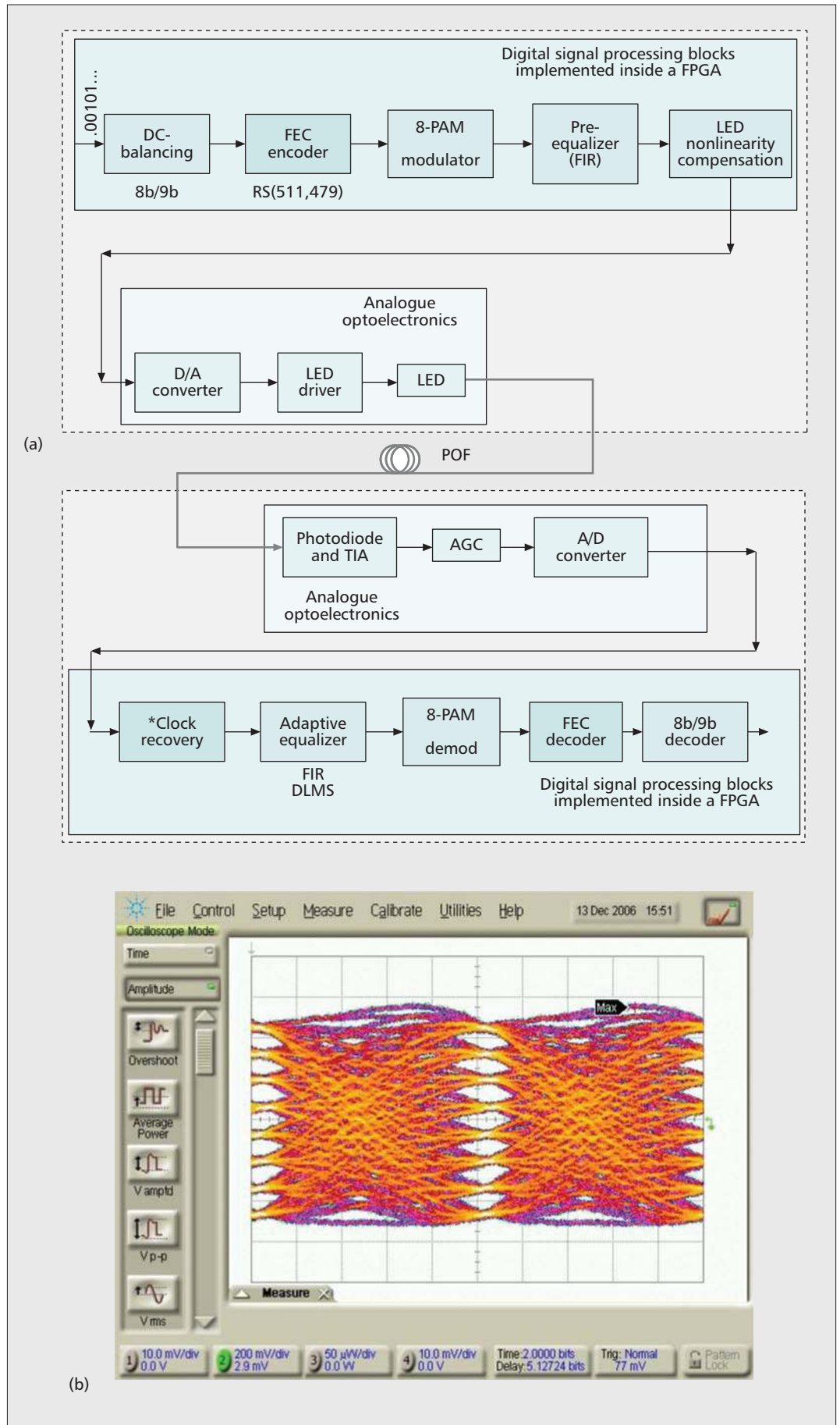
■ Figure 2. a) System setup.
