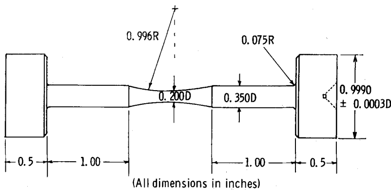
Fig. 2—Test-specimen dimensions
