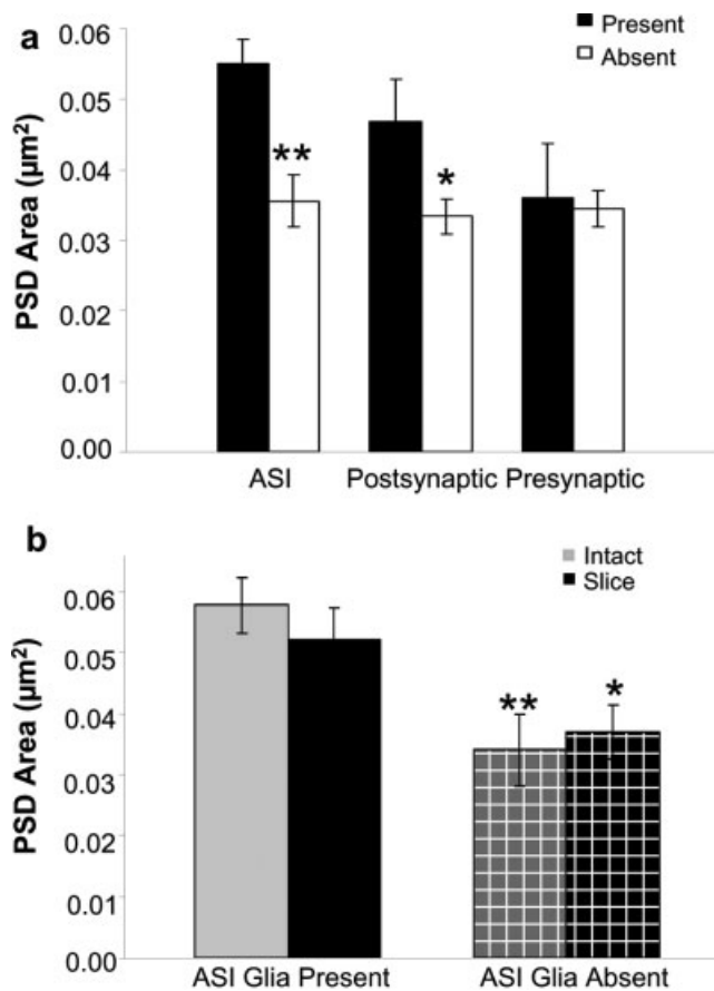
Fig. 4. Mean synapse size was larger for synapses with perisynaptic astroglia apposed to the ASI or postsynaptic spine. (a) Mean synapse size was larger when astroglia was present at the ASI ( 0.055 \pm 0.003 \mu\text{m}^2 ) than when it was absent ( 0.036 \pm 0.004 \mu\text{m}^2 ; **P < 0.0005 ). Mean synapse size was also greater when astroglia was present at the postsynaptic dendritic spine only ( 0.047 \pm 0.006 \mu\text{m}^2 vs. 0.033 \pm 0.002 \mu\text{m}^2 ; *P < 0.05 ). (b) Mean synapse size was larger when perisynaptic astrocyte was present at the ASI in both the intact ( **P < 0.005 ) and sliced ( *P < 0.05 ) hippocampus.
