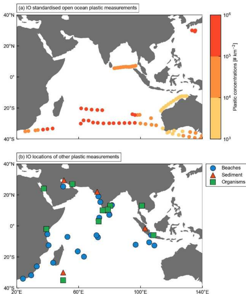
995 Figure 2. (a) Standardised measured concentrations of plastics in the Indian Ocean. Original samples were performed by Morris (1980); Reisser et al., (2013); Eriksen et al., (2014); Cózar et al. (2014) and were standardised by van Sebille et al., (2015). (b) Locations of plastic samples taken on beaches, in sediment, and in organisms around the Indian Ocean (references to individual studies listed in Table 1). Because sampling methods vary widely between studies, a quantitative comparison of measured plastic concentrations between these studies is not possible.
