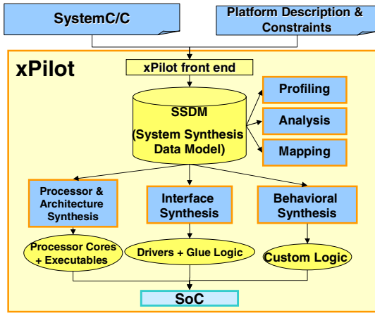
Fig. 1. xPilot system-level synthesis framework.
