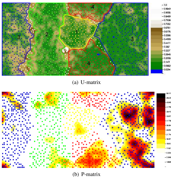
Fig. 5. Visualization maps of the highest-performing ESOM obtained and the 4 clusters identified. The 1365 best-matching neurons are drawn as squares on top of the maps. The maps illustrated are border-less since the map grid is organized in a toroid shape.
