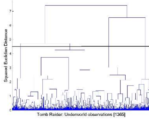
Fig. 3. Clustering of data using the Ward dendrogram method. A T value of 4.5 (illustrated with a horizontal black line) reveals 4 clusters.
