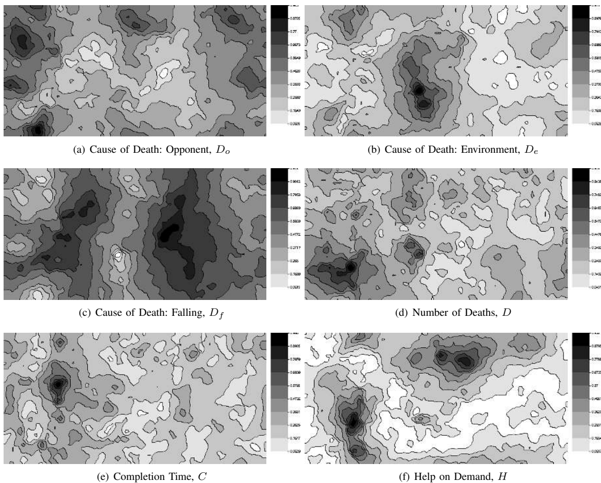
Fig. 6. The six component plane representations of the highest performing ESOM. The darker the area the higher the value of the component (feature).
