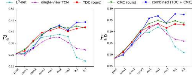
Figure 5: Cycle-consistency evaluation considering different embedding spaces. We compare naive l_2 pixel loss to temporal methods (TDC and single-view TCN) and cross-modal methods (CMC and L^3 -Net). Combining TDC and CMC yields the best performance for both 2 and 3-cycle-consistency, particularly at deeper levels of abstraction (e.g. no performance loss using FC1 or FC2).
