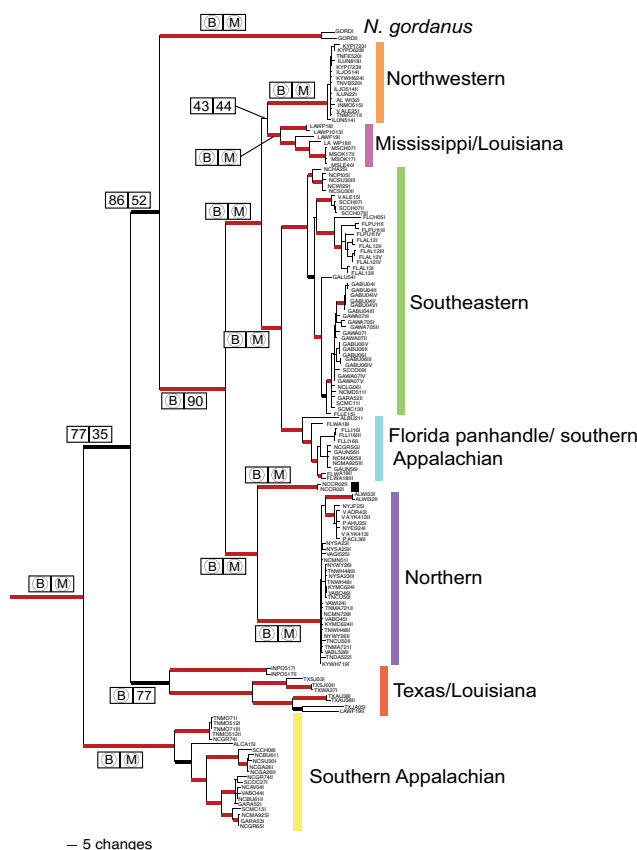
Figure 2 Inferred mtDNA haplotype phylogeny for Narceus using Bayesian inference. For major nodes, support values are represented in boxes. B and M represent posterior probabilities = 0.95 and maximum likelihood bootstrap values = 95%, respectively; PP and ML bootstrap values < 0.95 and 95% are represented by numbers in respective boxes. Thick red and thick black branches indicate PP = 1.00 and 0.70 – 0.95, respectively.
