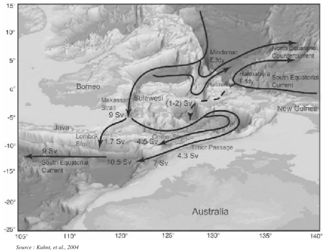
Figure 24. Throughflow of Indonesian sea current
