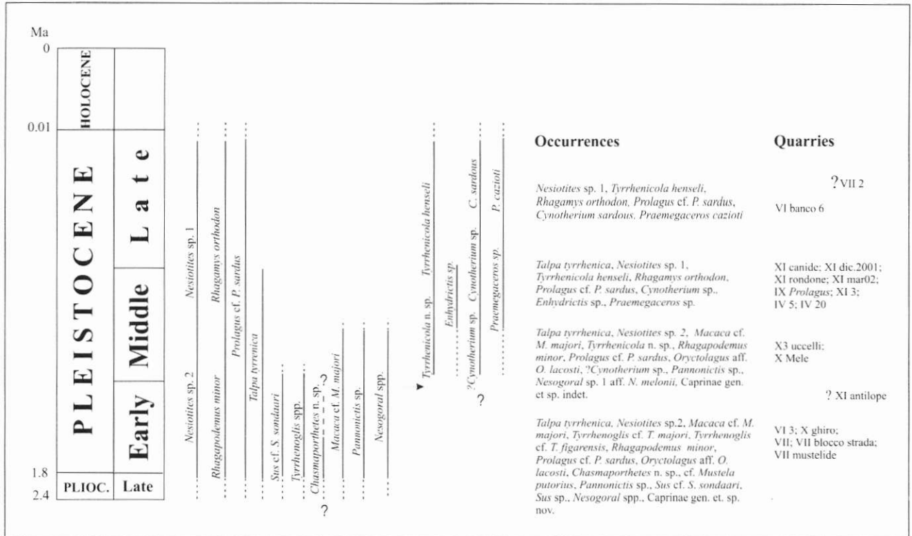
Fig. 16 - Chronological sequence of quarries of Monte Tuttavista and chronological range of mammal taxa documented in the fissure infillings.
