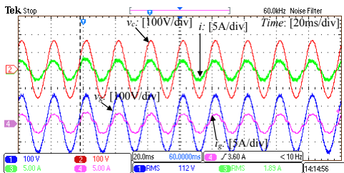
Figure 9. Operation under dc input voltage change from 200 V to 220 V
