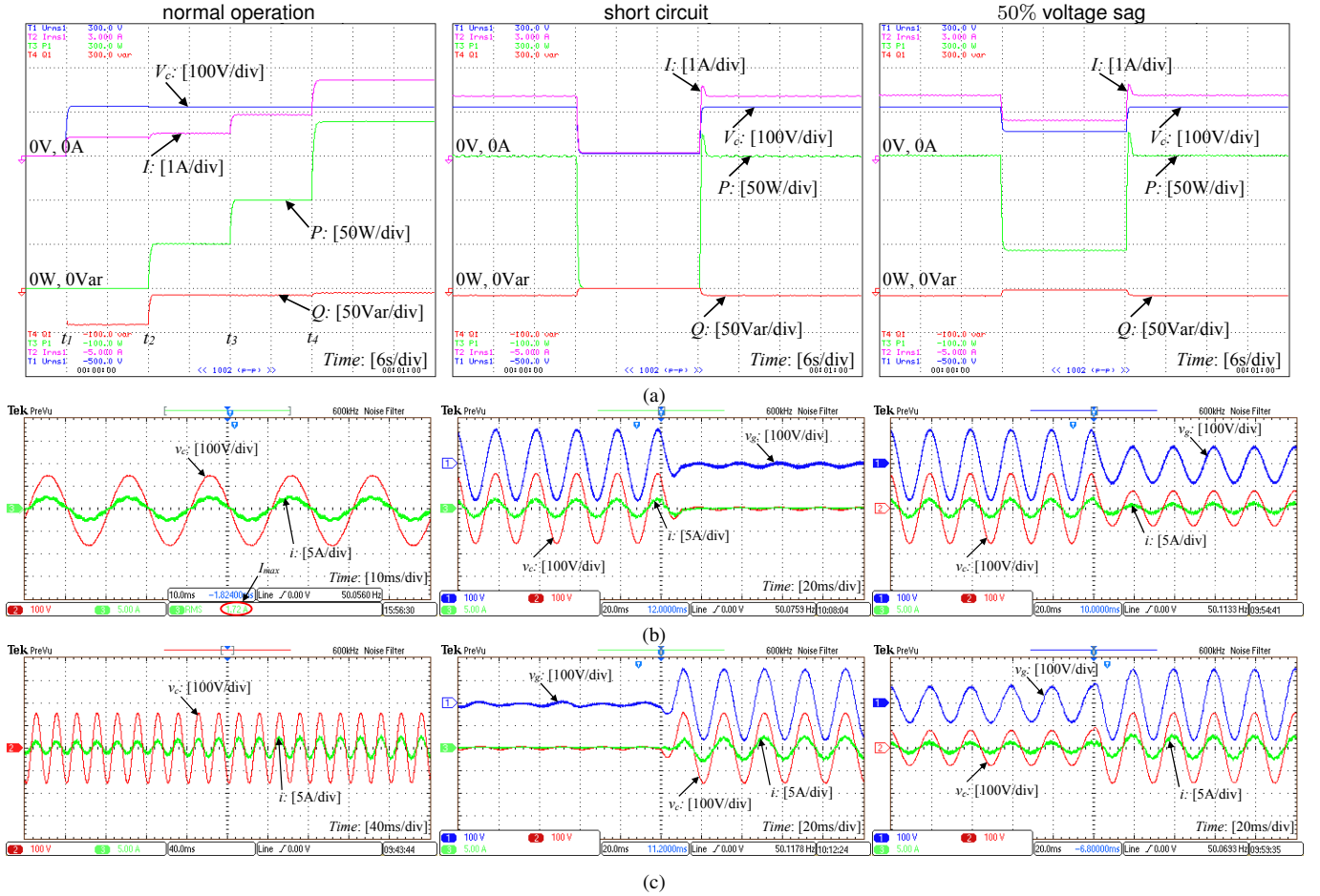
Figure 7. Operation under normal grid: (a) time response of the real, reactive power, capacitor voltage and inverter current, (b) steady-state response, (c) transient response around time instant t_4 (left column). Operation under grid faults: (a) time response of the real, reactive power, capacitor voltage and inverter current, (b) transient response when the fault occurs, (c) transient response when the fault is cleared (middle column: short circuit of the grid voltage, right column: 50% grid voltage sag)
