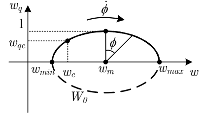
Figure 2. Phase portrait of the controller dynamics
