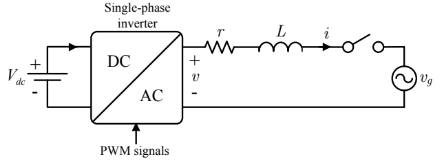
Figure 1. A single-phase grid-tied inverter with an L filter
