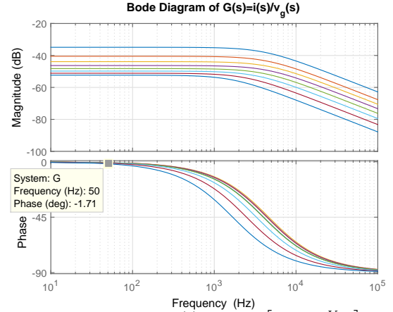
Figure 5. Bode plot of G(s) = \frac{i(s)}{v_g(s)} for w \in [w_{min}, \frac{V_g}{\tilde{I}_{min}}]
