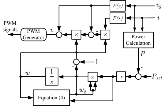
Figure 4. Proposed controller implementation
