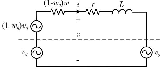
Figure 3. Closed-loop system equivalent circuit
