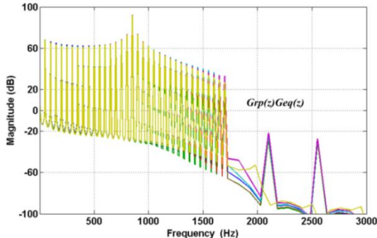
Fig. 11. Open loop gain G_{rp}(z)G_{eq}(z) amplitude response.
