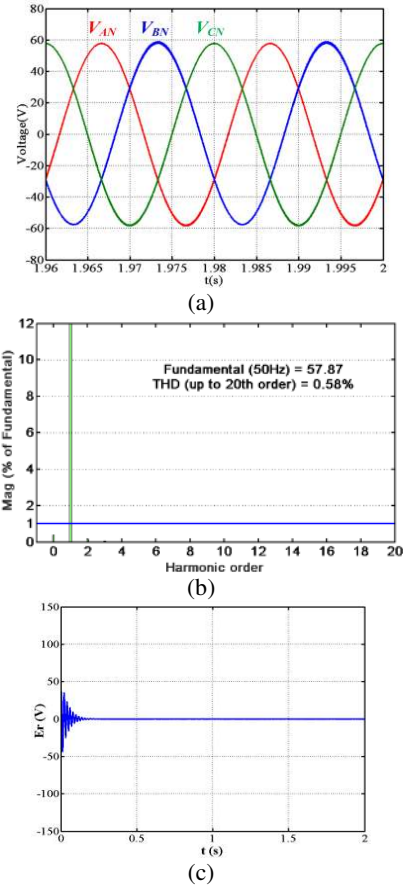
Fig. 14. FSTP-SQZS inverter using the proposed repetitive control scheme including S(z) and K_r=0.8 : (a) output phase voltage waveforms; (b) fundamental magnitude and low order harmonic distribution for phase A output voltage; and (c) error convergence process.
