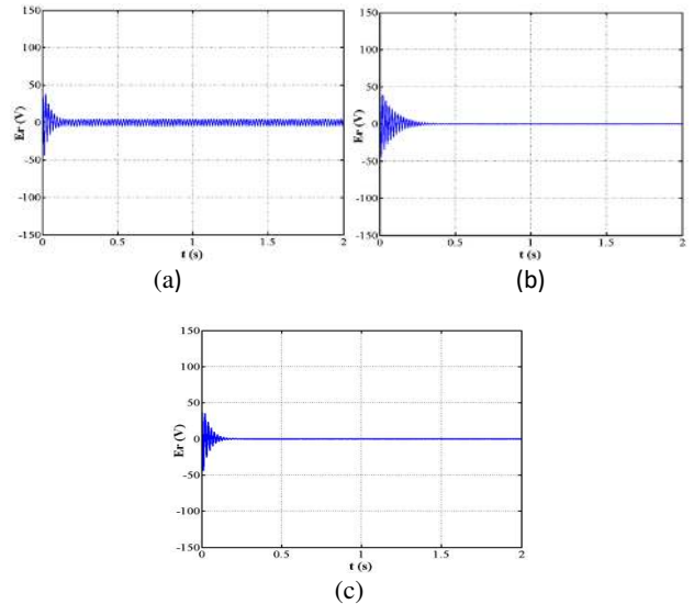
Fig. 15. Error convergence comparison for the plug-in repetitive controller with different parameters: (a) Q(z)=0.95 , K_r=0.8 , (b) Q(z) is low-pass filter, K_r=0.4 , and (c) Q(z) is low-pass filter, K_r=0.8 .
