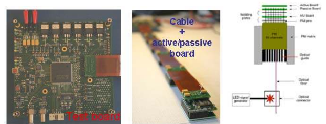
Fig. 7. Left: PMF test board. Center: kapton cable with 5 couples active-passive boards. Right: LED test set-up.
