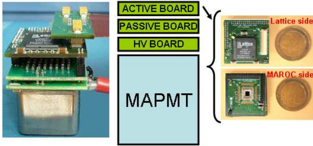
Fig. 4. PMF schematic and picture.
