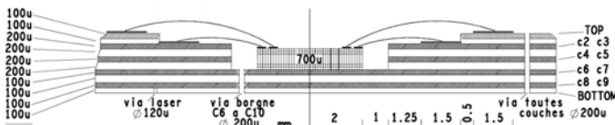
Fig. 5. Schematic view of the active board layer structure.
