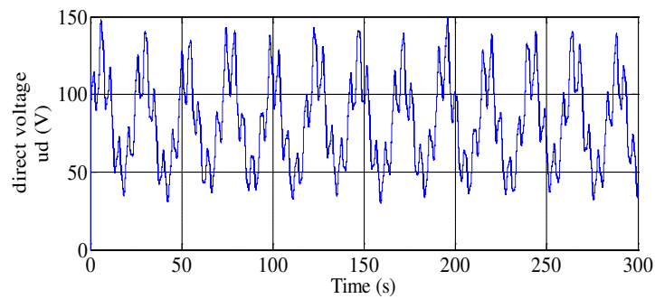
Figure 14. Voltage component u_d .
