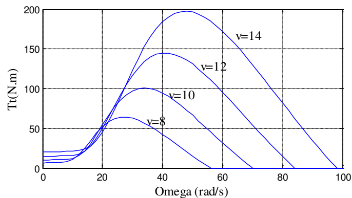
Figure 5. Curve family of aerodynamic torque versus \omega and v .
