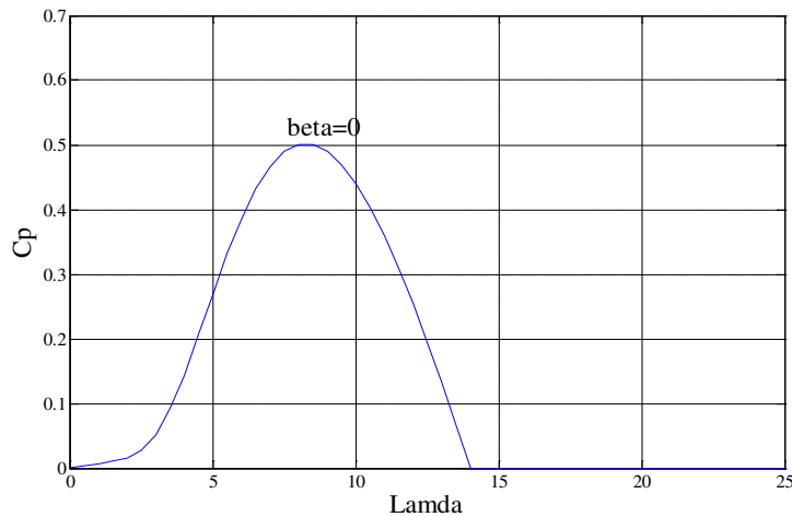
Figure 3. Power coefficient with different values of \lambda (with \beta = 0 ).
