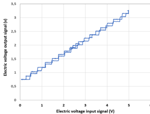
Fig. 7. Hysteresis curve
