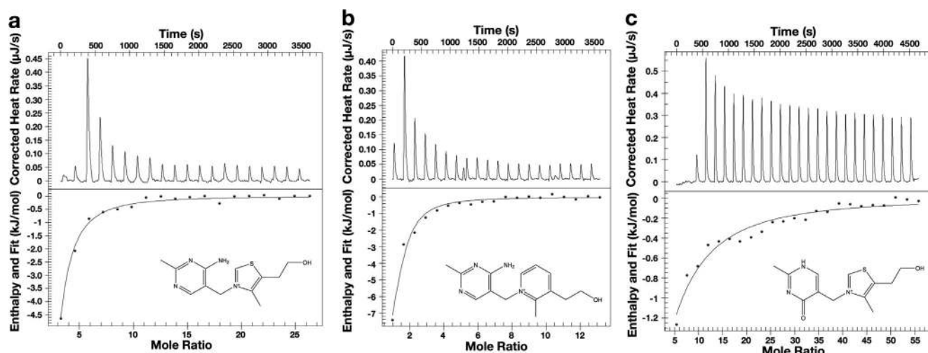
Figure 3. Substrate binding to PnuT sw . (a–c) Examples of isothermal titration calorimetry experiments showing (a) thiamine, (b) pyriothiamine, and (c) oxythiamine binding to PnuT sw .
