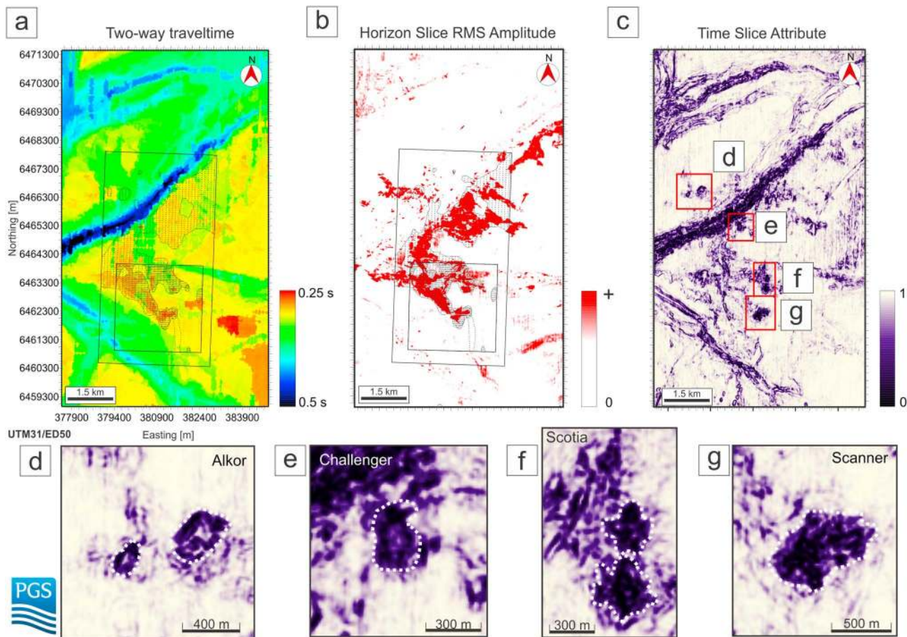
Figure 9. 3-D seismic horizon top S1.2/bottom S2. The horizon is given in (a) two-way traveltimes, (b) root-mean-square (RMS) amplitude horizon slice over a time window of \pm 50 ms across the unconformity between units S1.2 and S2 to map the fluids, and (c) symmetry attribute time slice. The slices show the gas accumulation within S2 across stratigraphic highs in between tunnel valleys in comparison to the previous analyses by Judd et al. (1994; see map inset in (a) and (b)). Below are shown close-ups of the symmetry attribute for the (d) Alkor, (e) Challenger, (f) Scotia, (g) Scanner pockmark complexes (Class 1 pockmarks). White dashed lines outline the pipe structures in the subsurface. The locations of (a), (b), and c are given in Figure 1.
