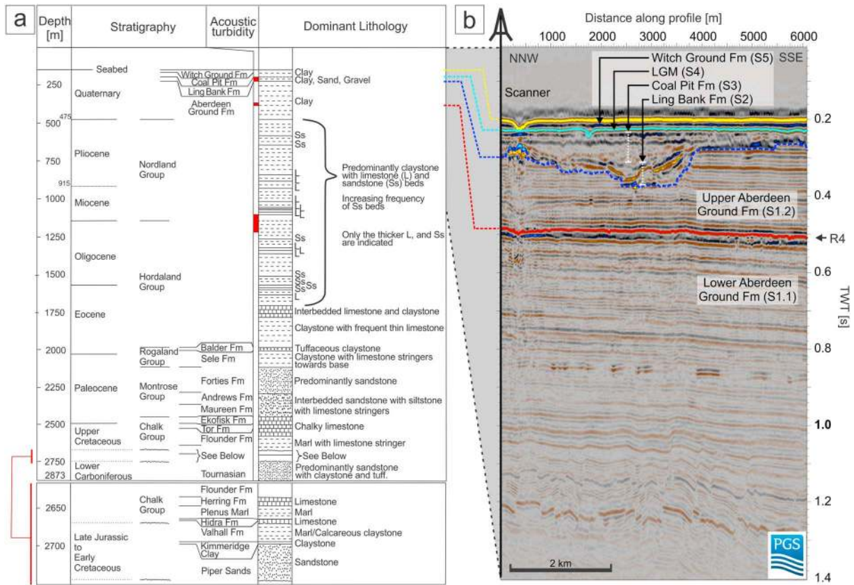
Figure 2. (a) Stratigraphic and lithological summary of well 15/25b-1A, located 400 m northwest of the western Scanner pockmark (modified after Judd et al., 1994). (b) 6-km-long representative seismic profile from conventional 3-D seismic data from north-northwest to south-southeast. The seismic profile shows major stratigraphic units lower Aberdeen Ground Formation (S1.1), R4 reflector, upper Aberdeen Ground Formation (S1.2), Ling Bank Formation (S2), Coal Pit Formation (S3), last glacial maximum deposits (LGM, S4) and the Witch Ground Formation (S5). The image shows distance along profile on the x axis and two-way traveltme (TWT) on the y axis. 1.4 s TWT correspond to a minimum depth of 1,050 m (at 1,500 m/s seismic velocity). The location of the profile is given in Figure 1.
