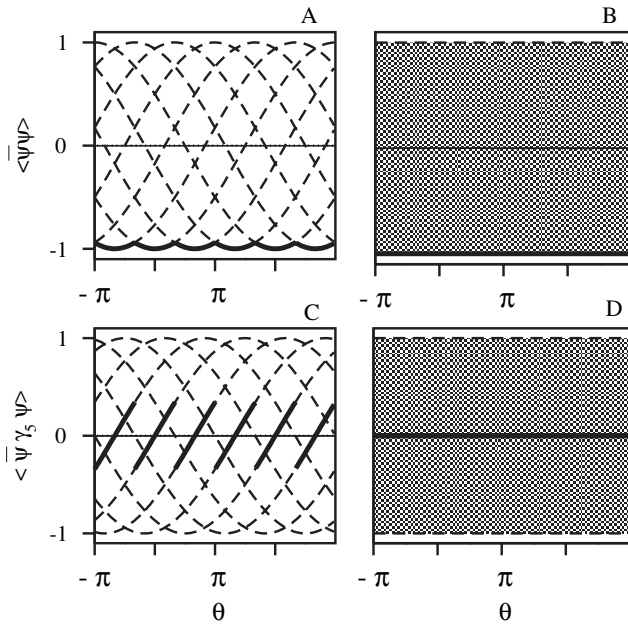
FIG. 1. The scalar (A and B) and pseudoscalar (C and D) quark condensates as functions of \theta for N_f = 3 in units of \aleph . The plots A and C are for rational q = 0.15 , while B and D correspond to any irrational q , for instance to q = \frac{3}{2.02\pi^2} = 0.15047\dots which is numerically only slightly different from 0.15. The dashed lines in A and C correspond to discrete minima of the free energy density which are degenerate for m \equiv 0 . The solid bold lines denote the minimum which is chosen by an infinitesimally small mass term for a given \theta . Points on the solid line in A, where two dashed lines cross each other, correspond to critical values of \theta , at which CP is broken spontaneously. This is signalled by the discontinuity in the pseudoscalar condensate in C. For irrational q , as illustrated in B and D, the dashed lines densely cover the strip between 1 and -1 , and the set of critical values of \theta turns out to be dense in \mathbb{R} . As will be discussed in the last section, an analogy can be seen between A (C) and motion on a torus over a closed trajectory, while a manifestation of the Poincaré recurrence theorem resulting in dense winding of a torus (for example, see [16]) can be recognized in B (D).
