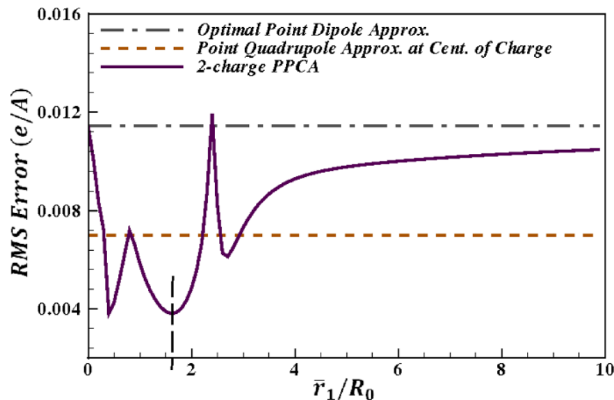
Figure 4. Accuracy of the 2-charge practical point charge approximation (PPCA) as a function of the distance \bar{r}_1 from the center of charge. For the sample charge distribution shown in figure 3. Accuracy is calculated as the RMS error, relative to the exact computation, at a distance of 2R_0 , where R_0 is the maximum extent of the charge distribution from the center of geometry. The point dipole and point quadrupole approximations with center of charge as the center of expansion are shown for comparison. The vertical dashed line represents the value \bar{r}_1 \approx 1.6R_0 that produces the lowest RMS error for the 2-charge PPCA in this case. Connecting lines are shown to guide the eye. doi:10.1371/journal.pone.0067715.g004
