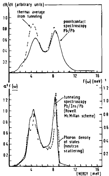
Fig. 16 Measured dR/dV point-contact spectrum of a lead micro-contact in a tunnel junction (after Yanson, 1974a). Resistance R_0 = 314 \Omega ; temperature T = 2.0 K. The phonon density of states F(\omega) (Stedman et al., 1967) and the Eliashberg function \alpha^2 F(\omega) (Rowell et al., 1973) are shown in the bottom part. The dashed line in the top part is the thermal average of the function \alpha^2 F(\omega) due to the bath temperature T = 2.0 K.
