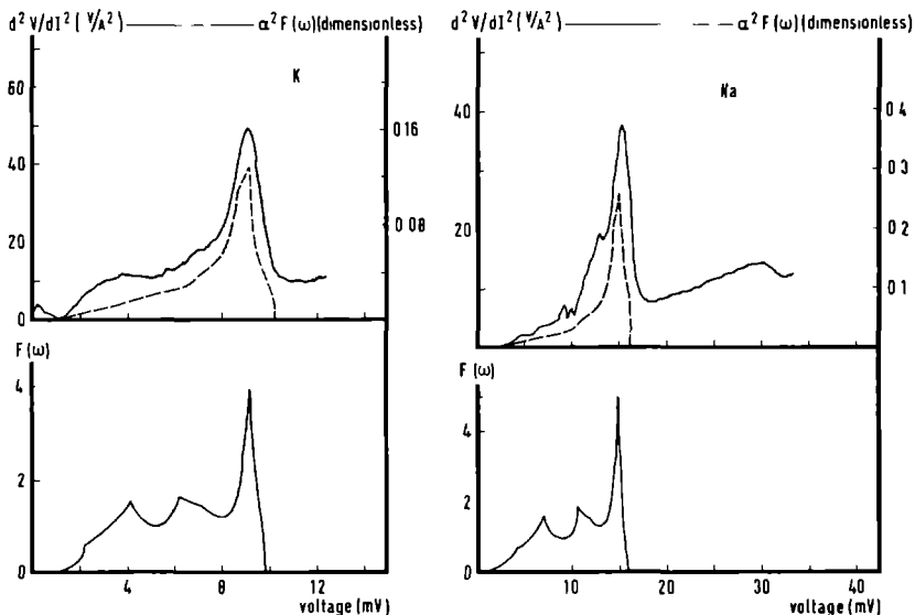
Fig. 18 Measured d^2V/dI^2 spectra for point contacts of potassium (left) and sodium (right). K point contact with resistance R_0 = 2.9 \Omega and at temperature T = 1.2 K; Na point contact with R_0 = 1.1 \Omega and at T = 1.5 K. The dashed curves are the theoretically obtained \alpha^2F -functions (Carbotte and Dynes, 1968). The bottom figures give the phonon density of states from neutron-scattering experiments (Cowley et al., 1966; Gilat and Raubenheimer, 1968).
