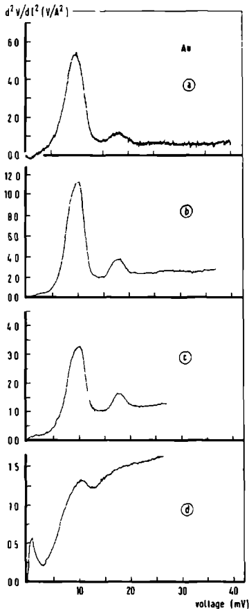
Fig. 22 Measured d^2V/dI^2 spectra for different gold point contacts (pressure type) with resistances R_0 = 2.4 \Omega (a), 0.7 \Omega (b), 0.4 \Omega (c) and 0.15 \Omega (d), at a temperature T = 1.2 \text{ K} .
