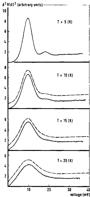
Fig. 26 Measured d^2V/dI^2 spectra at a temperature between 5 and 20 K for a Au point contact with resistance R_0 = 5.1 \Omega . The dashed lines (vertically shifted by one scale division) give the calculated thermal average using the measured spectrum at 5 K.
