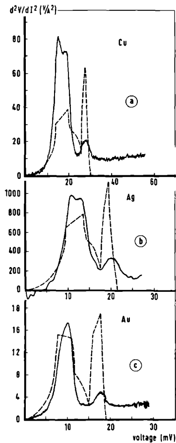
Fig. 17 Measured d^2V/dI^2 spectra of point contacts of the noble metals. Copper contact (a) with resistance R_0 = 3.3 \Omega and at temperature T = 1.5 K; silver contact (b) with R_0 = 16.3 \Omega and at T = 1.2 K; gold contact (c) with R_0 = 3.3 \Omega and at T = 1.2 K. The broken curves give the phonon densities of states F(\omega) obtained from neutron-scattering experiments (Lynn et al., 1973).
