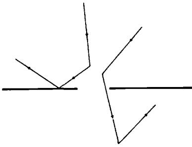
Fig.2 Point-contact in the Knudsen limit ( l > a ) leading to a ballistic transport of the electrons.
