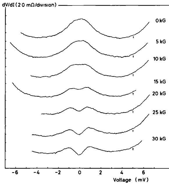
Fig. 3 : Magnetic field dependence of the differential resistance dV/dI of a Au-0.1 at.% Mn point contact as function of the applied voltage ( R = 2.5 \Omega ; T = 1.5 \text{ K} ). The curves are shifted with respect to the reference point indicated by ( \uparrow ).
