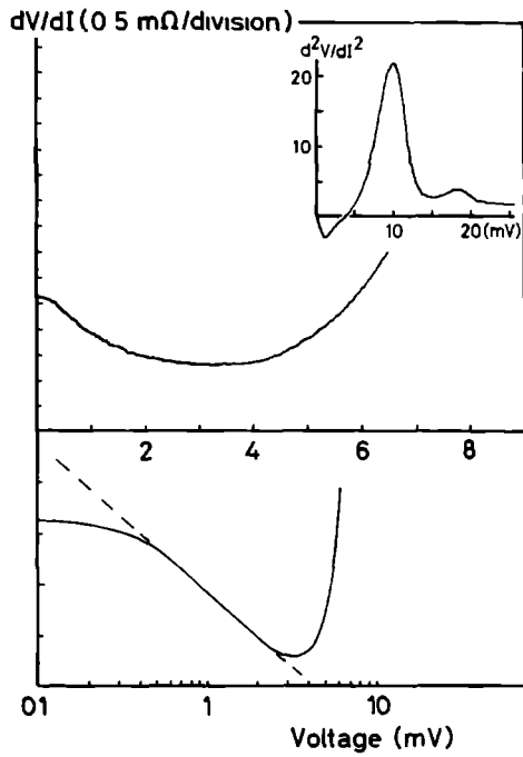
Fig. 1 : Differential resistance dV/dI of a Au-0.03 at.% Mn point contact as a function of the applied voltage on a linear and a logarithmic scale ( R=2.1\Omega ; T = 1.5 K). The dashed line gives the theoretically expected logarithmic behaviour. The inserted d^2V/dI^2 -curve indicates the well known typical point contact behaviour with the phonon peaks for Au at 10 and 18 mV.
