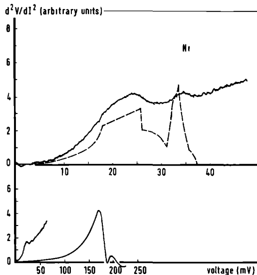
Fig. 29 Measured d^2V/dI^2 spectra for point contacts of Ni at a temperature T = 1.5 K. Top figure: resistance R_0 = 6.5 \Omega ; bottom figure. R_0 = 2.9 \Omega . The dashed line gives the phonon density of states obtained from inelastic neutron-scattering experiments (Birgeneau et al., 1964). In the bottom figure the singularity around 190 mV is shown together with the expanded signal at low voltages (phonon structure).
