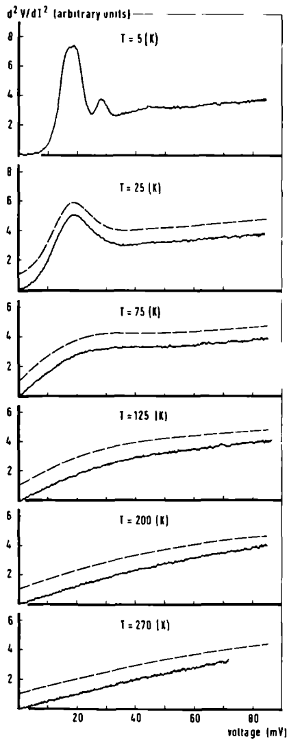
Fig. 27 Measured d^2V/dI^2 spectra at a temperature between 5 and 270 K for a Cu point contact with resistance R_0 = 1.7 \Omega at 5 K. The dashed lines (vertically shifted one scale division) give the calculated thermal average using the measured spectrum at 5 K.
