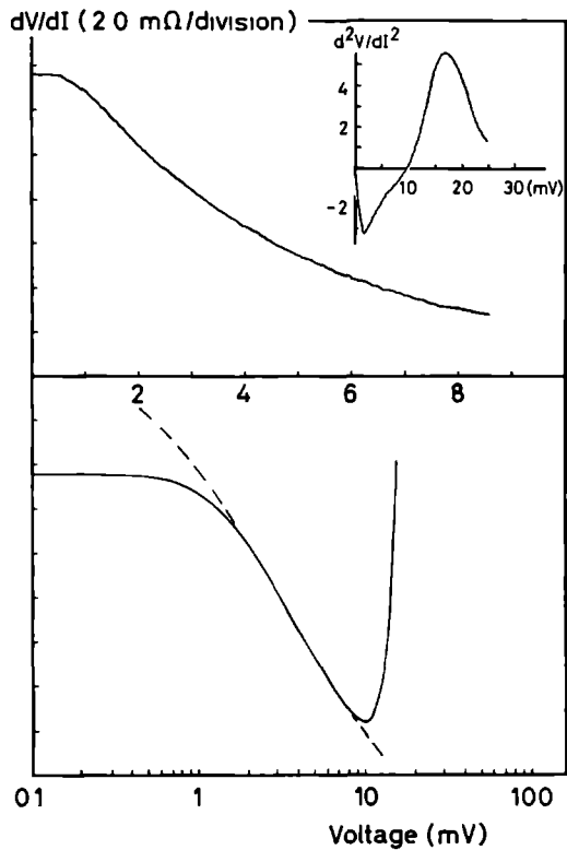
Fig. 2 : Differential resistance dV/dI of a Cu-0.1 at.% Fe point contact as function of the applied voltage on a linear and a logarithmic scale ( R = 1.2 \Omega ; T = 1.5 \text{ K} ). The dashed curve is the fitted Hamann-function with k_{\text{B}}T_{\text{K}} = 3.5 \text{ mV} and S = 0.5 . The inserted d^2V/dI^2 -curve indicates the well known typical point contact behaviour with the phonon peak for Cu at 17 mV.
