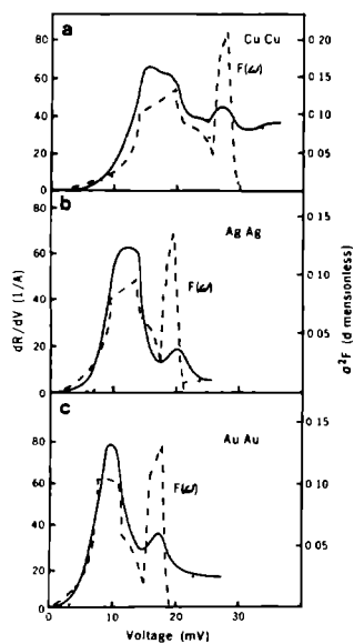
Fig. 2 (left) Photograph of the recorder sheet with (curve a) current I , (curve b) first derivative dI/dV and (curve c) second derivative d^2I/dV^2 plotted against applied voltage. Fig. 3 (right) The measured voltage derivative of the resistance of point contacts as function of applied voltage for (a) Cu, (b) Ag, and (c) Au is plotted as solid lines (left hand scale). The right hand scale is the derived value for \alpha^2 F . The background functions are shown as short dashed curves and the phonon density of states as long dashed curves.
