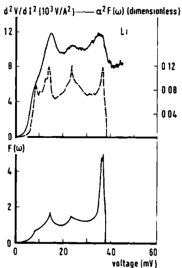
Fig. 19 Measured d^2V/dI^2 spectrum for a lithium point contact. Resistance R_0 = 25.4 and temperature T = 1.5 K. The dashed curve is the theoretically obtained \alpha^2 F -function (Hayman and Carbotte, 1971). The bottom figure gives the phonon density of states from neutron-scattering experiments (Smith et al., 1968).
