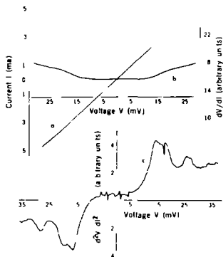
Fig. 2 (left) Photograph of the recorder sheet with (curve a) current I , (curve b) first derivative dI/dV and (curve c) second derivative d^2I/dV^2 plotted against applied voltage. Fig. 3 (right) The measured voltage derivative of the resistance of point contacts as function of applied voltage for (a) Cu, (b) Ag, and (c) Au is plotted as solid lines (left hand scale). The right hand scale is the derived value for \alpha^2 F . The background functions are shown as short dashed curves and the phonon density of states as long dashed curves.
