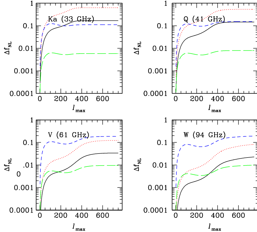
FIG. 8 (color online). The WMAP estimator bias terms \Delta f_{NL}^\alpha as a function of \ell_{\max} for radio point source density modulation (solid, black line); SZ number density modulation (dotted, red line); radio point source gravitational lensing magnification modulation (dashed, blue line); and SZ gravitational lensing magnification modulation (long-dashed, green line) in Ka – 33 GHz (upper left); Q – 40 GHz (upper right); V – 61 GHz; and W – 94 GHz. The density modulation terms produce a negative bias, while the magnification bias produce a positive bias.
