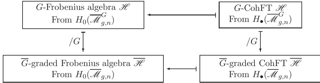
FIGURE 1. Schematic of Question 1 where each box contains an algebraic structure and the responsible homology group, the horizontal arrows are restrictions, and the vertical arrows are ‘quotients’ by G . When G is the trivial group, the two rows coincide.
