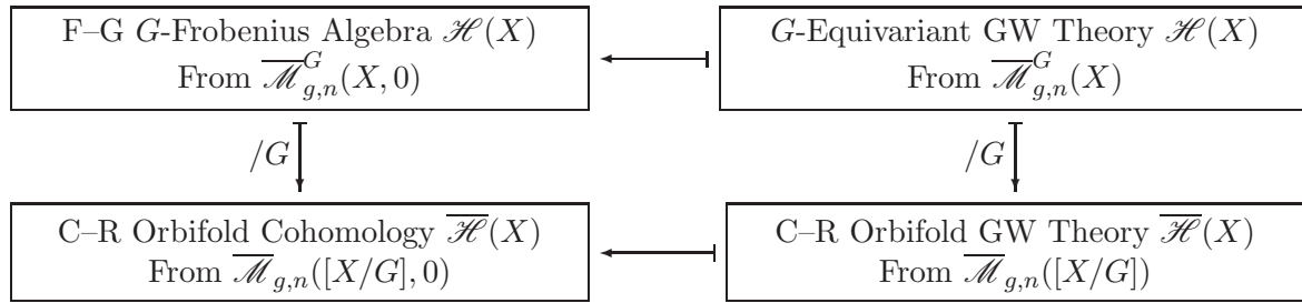
FIGURE 2. Schematic of Question 2 where each box contains an algebraic structure and the relevant moduli space, F–G denotes Fantechi–Göttsche, C–R denotes Chen–Ruan, the horizontal arrows denote restriction, and the vertical arrows denote taking ‘quotients’ by G .
