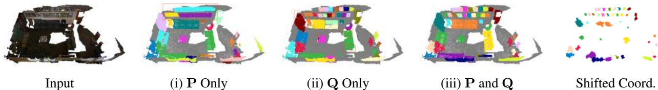
Figure 4: Instance predictions produced by models trained with clustering on (i) P only, (ii) shifted coordinates Q only, and (iii) both. The last column shows the predicted instances of (iii) represented with Q, where stuff points are ignored.
