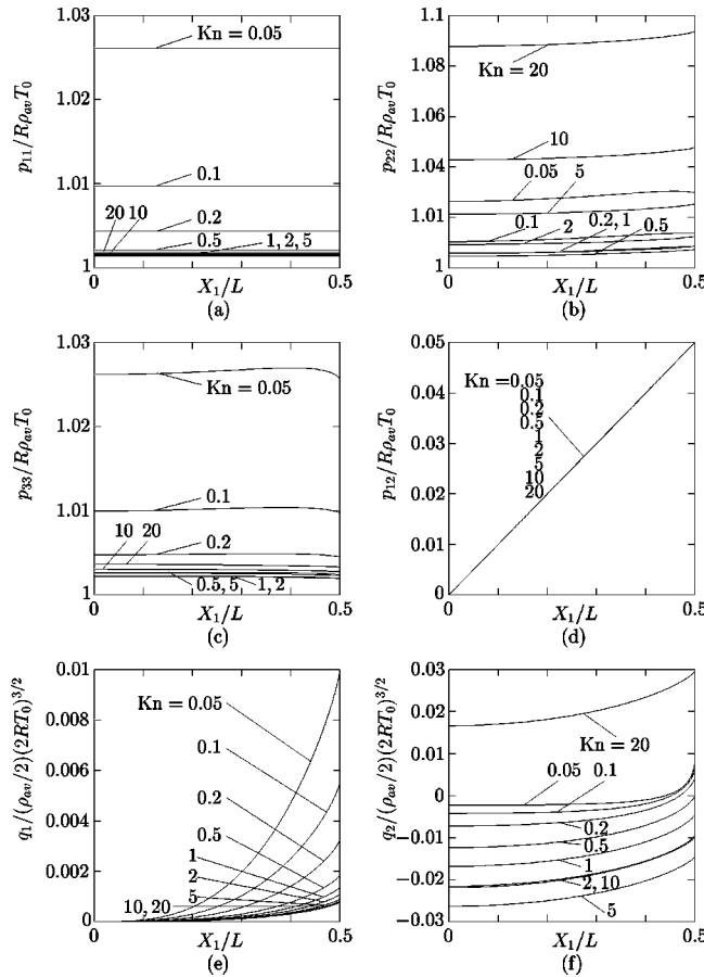
FIG. 13. The profiles of the nontrivial components of the stress tensor p_{ij} and the heat-flow vector q_i for various Kn in the case of \hat{F}=0.05 . (a) p_{11} , (b) p_{22} , (c) p_{33} , (d) p_{12} , (e) q_1 , (f) q_2 .
