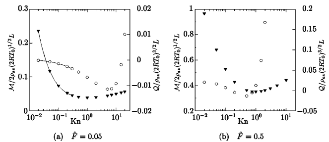
FIG. 15. The mass-flow rate \mathcal{M} and the heat-flow rate Q vs Kn. (a) \hat{F}=0.05 , (b) \hat{F}=0.5 . Here, \blacktriangledown indicates the mass-flow rate, \circ the heat-flow rate, and the solid line the corresponding results based on the asymptotic analysis in Sec. III.
