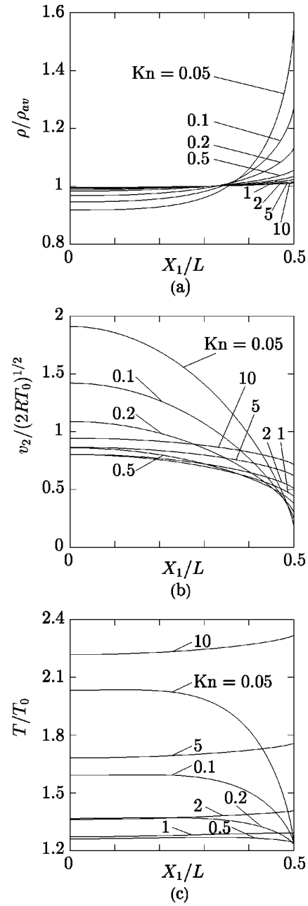
FIG. 12. The profiles of the density \rho , flow velocity v_2 , and temperature T for various \text{Kn} in the case of \hat{F}=0.5 . (a) \rho , (b) v_2 , (c) T .
