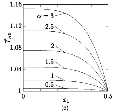
FIG. 1. The solution \hat{\rho}_{H0} , \hat{v}_{2H0} , and \hat{T}_{H0} for various \alpha . (a) \hat{\rho}_{H0} , (b) \hat{v}_{2H0} , (c) \hat{T}_{H0} .
