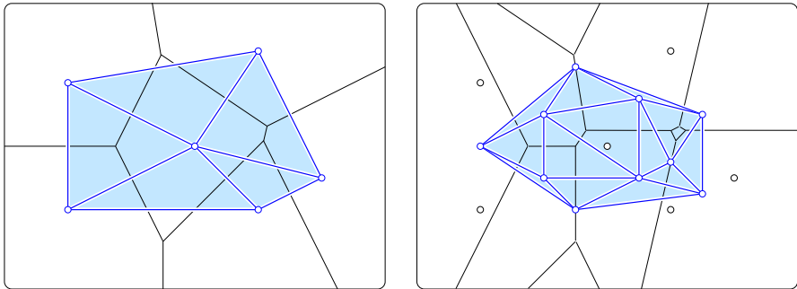
Fig. 2 The order-1 Delaunay mosaic on the left and the order-2 Delaunay mosaic on the right, both superimposed on their corresponding Voronoi tessellations
