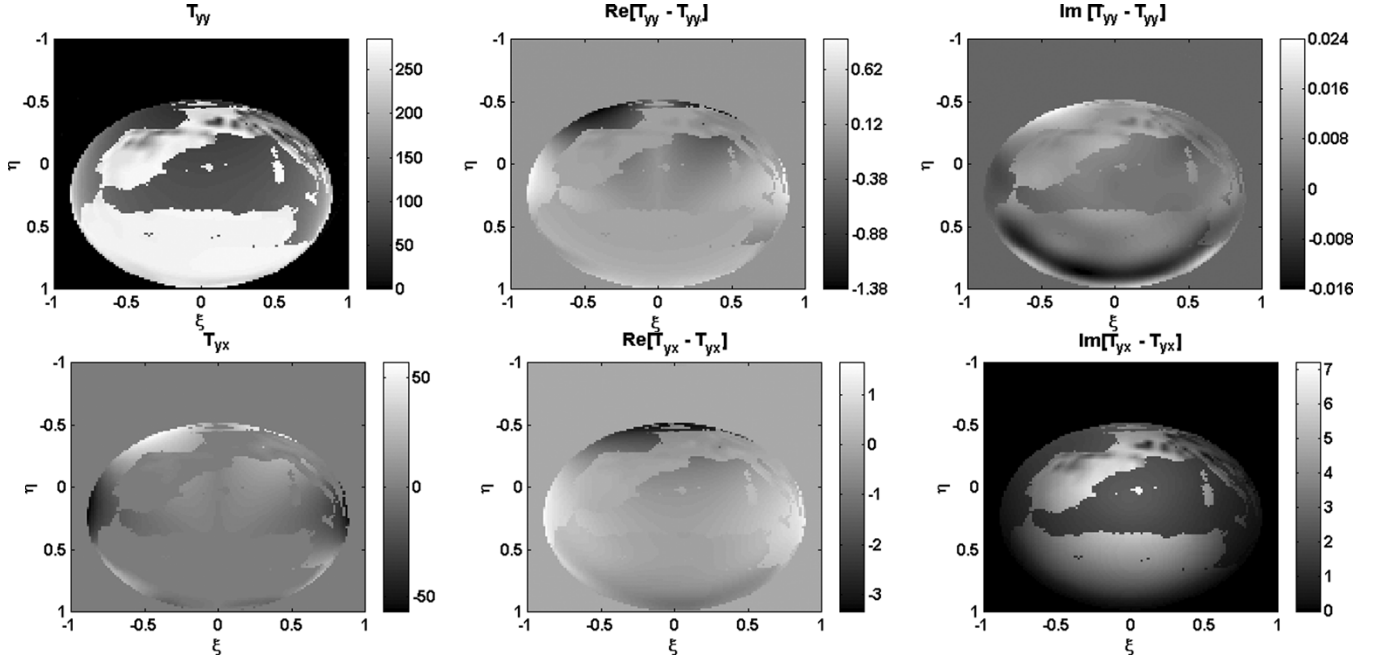
Fig. 1. Image errors maps in a high-contrast scene if antenna cross-polarization patterns are neglected: T_{yy} = A^2 T_{vv} + B^2 T_{hh} and T_{yx} = AB (T_{vv} - T_{hh}) . Root mean squared errors in the alias-free field of view: \sigma_{\text{Re}[\hat{T}_{xx}^{id} - \hat{T}_{xx}^{id}]} = 0.18 K, \sigma_{\text{Im}[\hat{T}_{xx} - \hat{T}_{xx}^{id}]} = 5.5 \cdot 10^{-3} K, \sigma_{\text{Re}[\hat{T}_{yy} - \hat{T}_{yy}^{id}]} = 0.15 K, \sigma_{\text{Im}[\hat{T}_{yy} - \hat{T}_{yy}^{id}]} = 3.6 \cdot 10^{-3} K, \sigma_{\text{Re}[\hat{T}_{yx} - \hat{T}_{yx}^{id}]} = 0.30 K and \sigma_{\text{Im}[\hat{T}_{yx} - \hat{T}_{yx}^{id}]} = 3.5 K.
