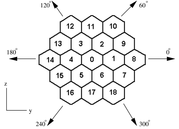
Fig. 1. The numbering system used for the Germanium SPI detectors. The 6 directions used in the polarisation analysis are shown along with the y - and z -coordinate axes of the spacecraft. The x -axis is normal to the detector plane.
