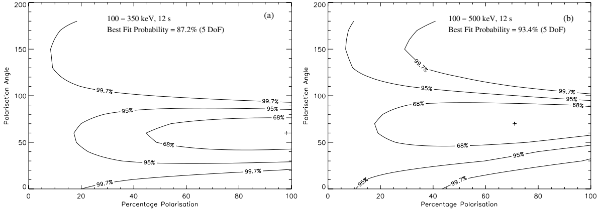
Fig. 9. Contour plots of the percentage polarisation as a function of the polarisation angle for the six scatter directions ( 0^{\circ} – 360^{\circ} ) in the 12 s interval, showing the 68%, 95% and 99.7% probability contours. The plots indicate a non-zero value for the level of polarisation. a) refers to the energy range 100–350 keV and b) refers to the energy range 100–500 keV.
