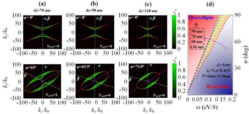
FIG. 8. (a)–(c) The top row shows the numerically simulated PTCs without rotation at the vacuum gap of 70, 90, and 110 nm at a frequency of 0.12 \text{ eV}/\hbar , respectively. The bottom row shows the PTCs at the rotation angle of topological transitions for the vacuum gap of 70, 90, and 110 nm, respectively. The red solid lines are the dispersion after hybridization of twisted hyperbolic system. The pink dashed lines are the dispersion after hybridization of twisted hyperbolic system. The blue dotted lines and the dotted dashed lines are the optical axis of the top grating (no rotation) and bottom grating (with rotation) of twisted bilayer system. (d) Topological transition regions as a function of frequency and rotation angles at different vacuum gap.
