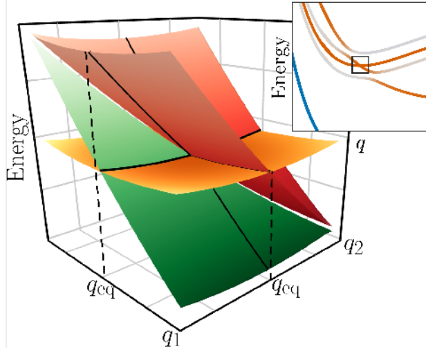
Figure 5: Zoom on the collective light-induced conical intersection between dark state PoPES under motion of two molecules.
