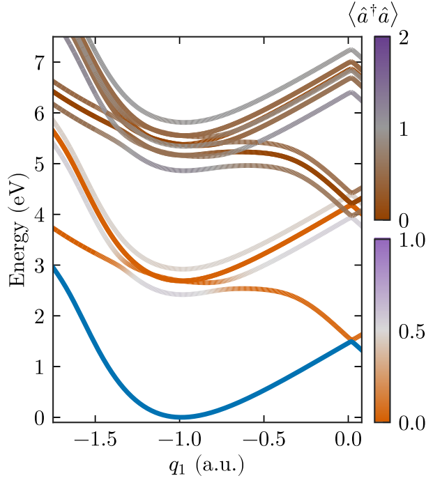
Figure 6: PoPES up to the two-excitation subspace for the model molecule of Fig. 2(c,d). The two color scales indicate the photon fraction in the single- and two-excitation subspace, respectively.
