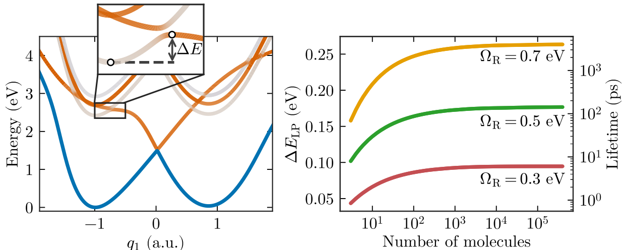
Figure 4: Collective protection effects: (a) PoPES for N = 50 molecules in strong coupling, one of which can move while the rest are frozen in their equilibrium position. The inset shows a zoom to the region where the effect of collective protection is most clearly seen. (b) Energy barriers vs number of molecules for different values of Rabi splitting. The right axis shows the equivalent lifetime predicted through transition state theory.
