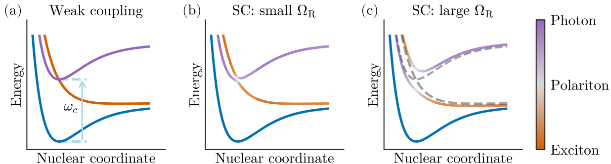
Figure 1: Conceptual potential energy surfaces for a single molecule and a light mode in (a) weak coupling and (b,c) strong coupling for different coupling strengths. The color represents the photonic fraction of the state from purely excitonic (orange) through polaritonic (light gray) to purely photonic (purple).
