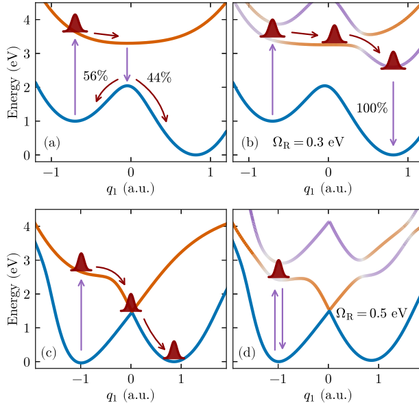
Figure 2: Polaritonic potential energy surfaces of two model molecules in weak and strong coupling. (a,c) Bare molecules without light-matter interaction. (c,d) Strongly coupled molecules, with (b) \Omega_R = 0.3 eV and (d) \Omega_R = 0.5 eV (photon energy \omega_c = 2.65 eV in both cases). The color scale is identical to Fig. 1.
