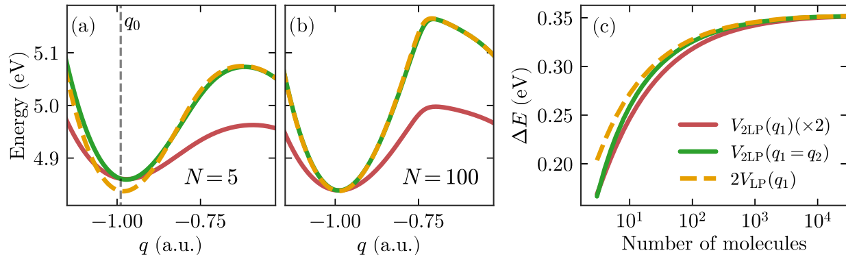
Figure 7: (a,b) Comparison of the PoPES in the double-excitation subspace for motion of one molecule (red line) and two molecules (green line), and twice the lower PoPES in the single-excitation subspace for motion of one molecule (orange dashed line), for N = 5 and N = 100 coupled molecules, respectively. (c) Dependence of the energy barrier for double photoisomerization with the number of molecules for the reaction paths corresponding to the PoPES in (a,b).
