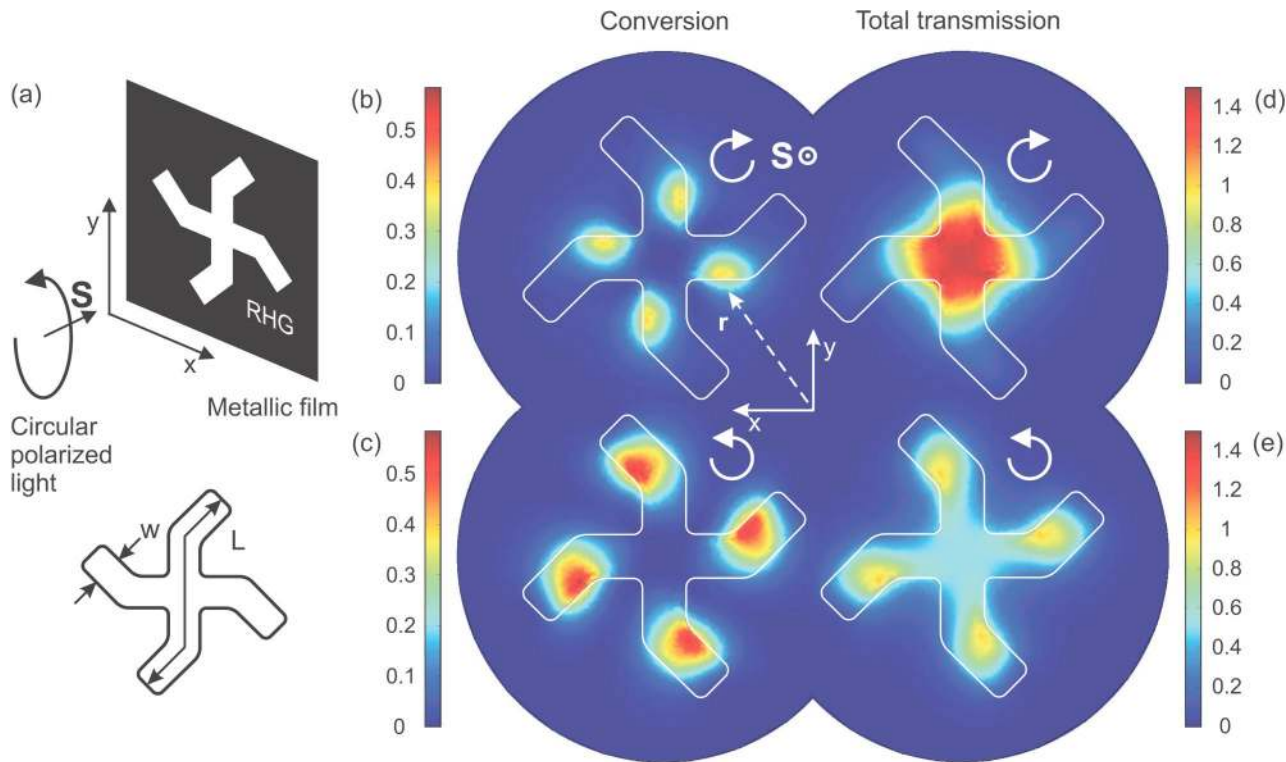
FIG. 1. (Color online) (a) General arrangement of the numerical simulations. Left field maps : Intensity [S_0^{tr}(\mathbf{r}) \pm S_3^{tr}(\mathbf{r})] / [2S_0^{in}(\mathbf{r})] of the polarization converted component of transmitted radiation for (b) RCP and (c) LCP incident waves. Right field maps : Intensity S_0^{tr}(\mathbf{r}) / S_0^{in}(\mathbf{r}) of total transmitted radiation for (d) RCP and (e) LCP incident waves. For all field maps, the incident wave propagates in the direction of the reader. The arrows illustrate the rotational direction of the electric field vector of the incident wave in the plane of the structure.
