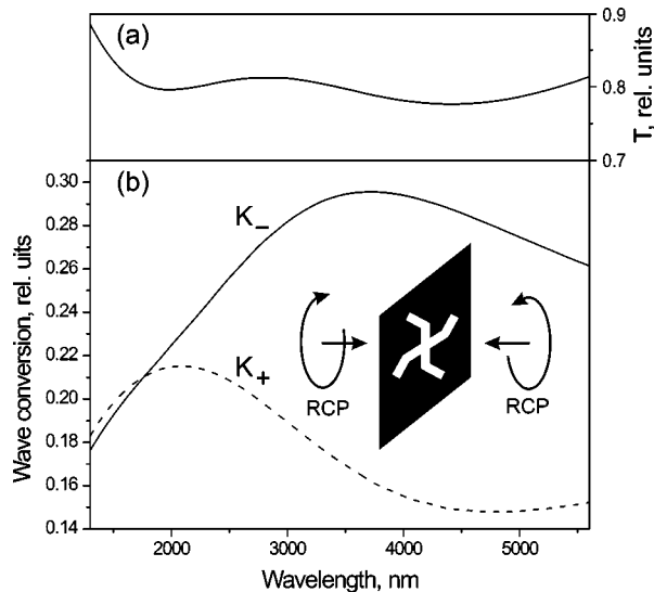
FIG. 2. (a) Wavelength dependence of the total transmission T through the gamadion opening; (b) wavelength dependence of the total polarization conversion efficiencies K_{\pm} for incident waves with the same (dashed line, K_+ ) and opposite (solid line, K_- ) handedness of the gamadion. Inset figure shows that the perceived sense of twist of a hole in a flat screen depends on from which side of the screen it is observed. The polarization conversion efficiency for a wave of a given handedness depends on whether it falls on the screen from one side or another.
