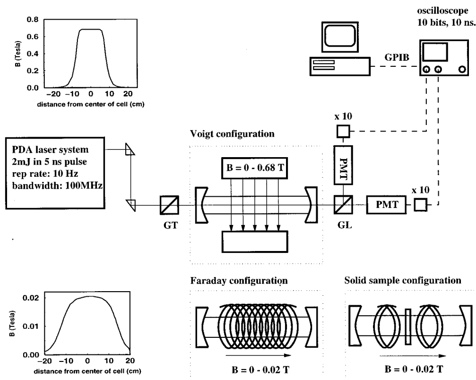
FIG. 1. Schematic view of the experimental setup. Pulsed narrow-band laser radiation is coupled into an optically stable ring down cavity. Prior to entering the cavity, the light passes through a Glan–Thompson polarizer (GT). The light exiting the cavity is split by a Glan–Laser polarizer (GL) into two mutually orthogonal polarized components that are recorded independently. The measured magnetic field strength along the axis of the cavity is indicated in the inset both for the Voigt and for the Faraday configuration. In the Faraday configuration for the solid sample, two Helmholtz coils are used to create the magnetic field.
