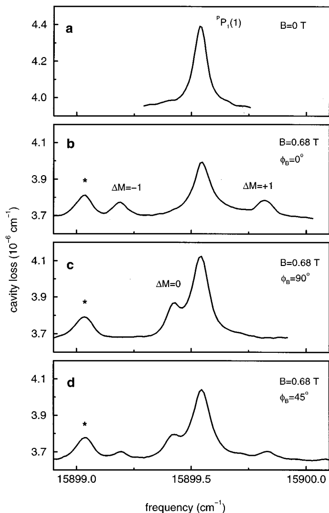
FIG. 3. The CRD absorption spectrum of the ^P P_1(1) line of the b^1\Sigma_g^+(v'=2) \leftarrow X^3\Sigma_g^-(v''=0) magnetic dipole transition in ^{16}\text{O}_2 , measured at a pressure of 420 mbar, without polarization selection in the detection step. In (a) no magnetic field is applied. In (b)–(d) a magnetic field of 0.68 T is applied in the Voigt configuration and the plane of polarization of the incoming light makes an angle \phi_B = 0^\circ , \phi_B = 90^\circ , and \phi_B = 45^\circ with the \mathbf{B} field, respectively. The line indicated with an asterisk is due to water absorption.
