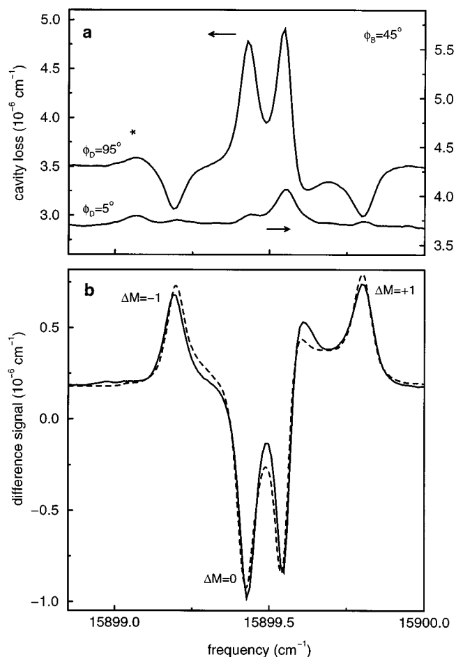
FIG. 4. The PDCRD spectrum of the ^P P_1(1) line of the b^1\Sigma_g^+(v'=2) \leftarrow X^3\Sigma_g^-(v''=0) transition in ^{16}\text{O}_2 , measured at a pressure of 400 mbar in the Voigt configuration, with \phi_B = 45^\circ . The polarization dependent cavity loss spectra shown in the upper part of the figure are recorded for \phi_D = 95^\circ and \phi_D = 5^\circ . In the lower part of the figure the difference between the two spectra, showing exclusively the effect of polarization-dependent absorption, is shown together with the simulated spectrum according to Eq. (7). The line indicated with an asterisk is due to water absorption.
