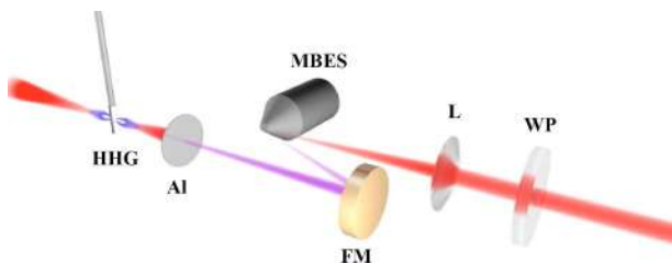
FIG. 2. (Color online) Schematic of the experimental setup. HHG, high harmonic generation; Al, Aluminum filter; MBES, Magnetic bottle electron spectrometer; WP, Retarding wave plate; L, Adjustable lens; FM, Gold focusing mirror.
