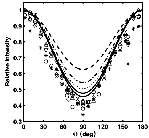
FIG. 3. Variation of the sideband intensity as a function of the relative angle \Theta between the polarization vectors of the XUV and the IR beams. Experimental data for different sidebands: (*)SB 14 , (◇)SB 16 , (▽)SB 18 , (Δ)SB 20 , and (○)SB 22 . Theoretical calculations: (--)SB 14 , (-)SB 16 , (·)SB 18 , (-)SB 20 , and (-)SB 22 .
