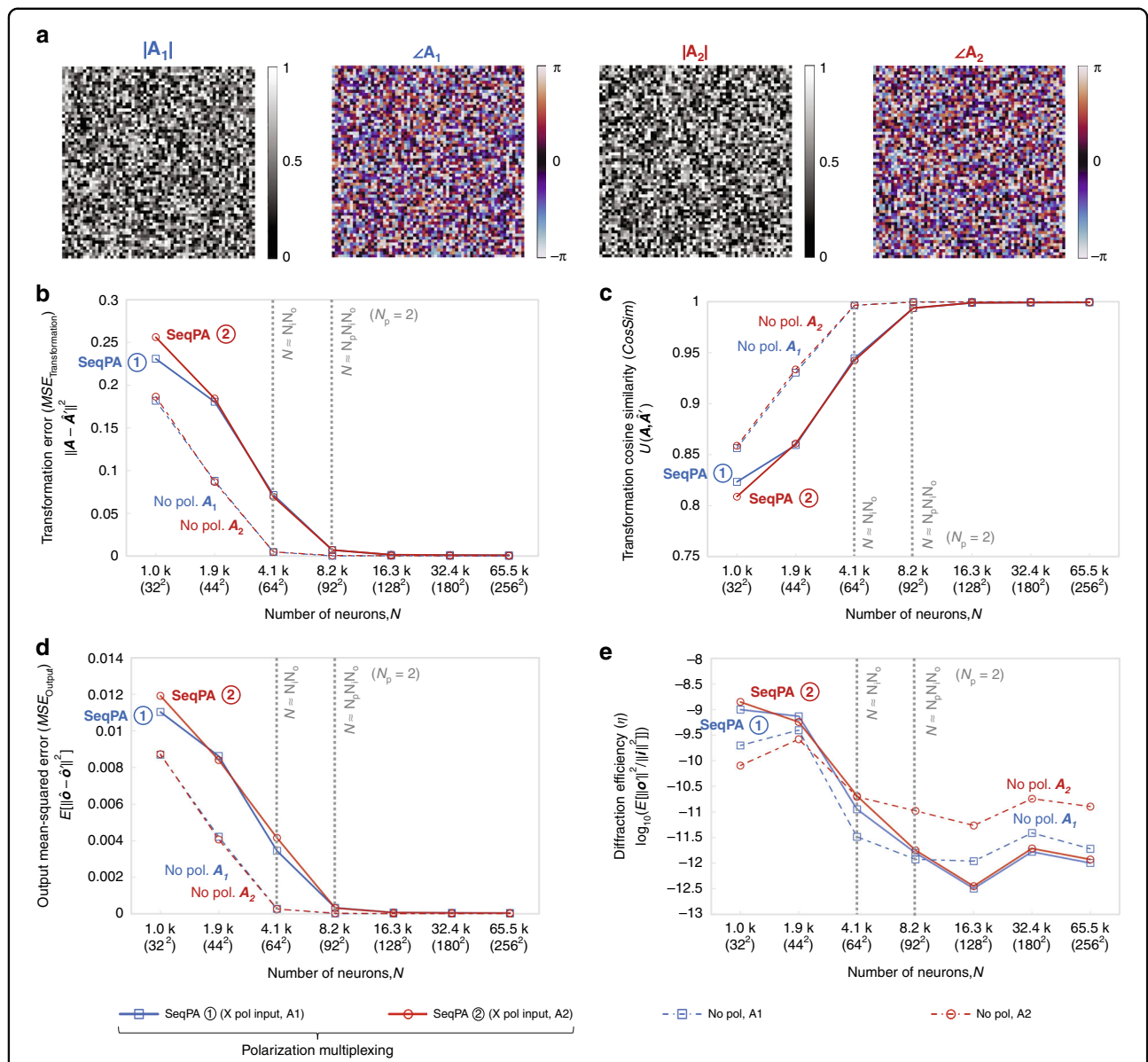
Fig. 2 Diffractive all-optical transformation results for 2-channel polarization multiplexing using the sequential polarization access (SeqPA) mode. a Amplitude and phase of the arbitrarily generated matrices A_1 and A_2 , which serve as the ground truth (target) for the diffractive all-optical transformations. b Curves representing the normalized mean-squared error between the ground truth transformation matrices ( A_1 and A_2 ) and the all-optical transforms ( \hat{A}_1 and \hat{A}_2 ) resulting from the trained diffractive networks as a function of the number of diffractive neurons N . The solid curves are achieved by the polarization-multiplexed diffractive networks trained using the SeqPA mode, which are compared with the dashed curves achieved by the regular diffractive networks trained with the same set of N but without any polarization multiplexing. For the polarization-multiplexed models, the results for the two polarization channels ① and ②, corresponding to transforms \hat{A}_1 and \hat{A}_2 , are shown in separate curves that are labeled with “SeqPA ①” and “SeqPA ②”, respectively. For the regular diffractive models without polarization multiplexing, the results for all-optical approximation of A_1 and A_2 are shown in separate curves labeled with “No pol. A_1 ” and “No pol. A_2 ”, respectively. The space between the simulation data points is linearly interpolated. c Same as (b) but the cosine similarity between the all-optical transforms and their ground truth shown in (a) is reported. d Same as (b) but the mean-squared error between the diffractive network output fields and their ground truth is reported. e Diffraction efficiency of the presented diffractive networks
