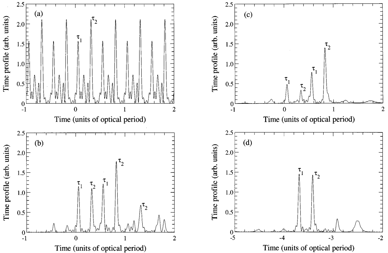
FIG. 3. Time profile |\bar{x}_F(t)|^2 calculated for a single neon atom and composed of the Fourier components with \Omega_{\min}=41\bar{\omega}\leq\Omega\leq\Omega_{\max}=61\bar{\omega} . The laser intensity is 4\times 10^{14} W/cm 2 , and the wavelength 825 nm. (a) Linear polarization, (b) time-dependent elliptical polarization with \Delta=\bar{\omega}/32 , (c) and (d) time-dependent elliptical polarization with \Delta=\bar{\omega}/16 .
