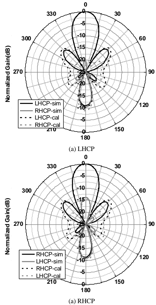
Fig. 15. Radiation patterns of the array antenna in XOZ plane.
