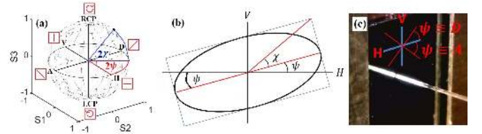
Fig. 2. Polarisation parameters. (a): Ellipticity ( \chi ) and major axis angles ( \psi ) on the Poincare sphere, with vertical ( V ), horizontal ( H ), diagonal ( D ) and anti-diagonal ( A ) \psi polarisations; (b) Polarization ellipse defining \psi and \chi (c) Wafer alignment with cleaved axis aligned to H , V (blue). The D , A example \psi values (red) show the degeneracy of \psi on the left and right sides of the diagram i.e. that \psi has a range of \pi .
